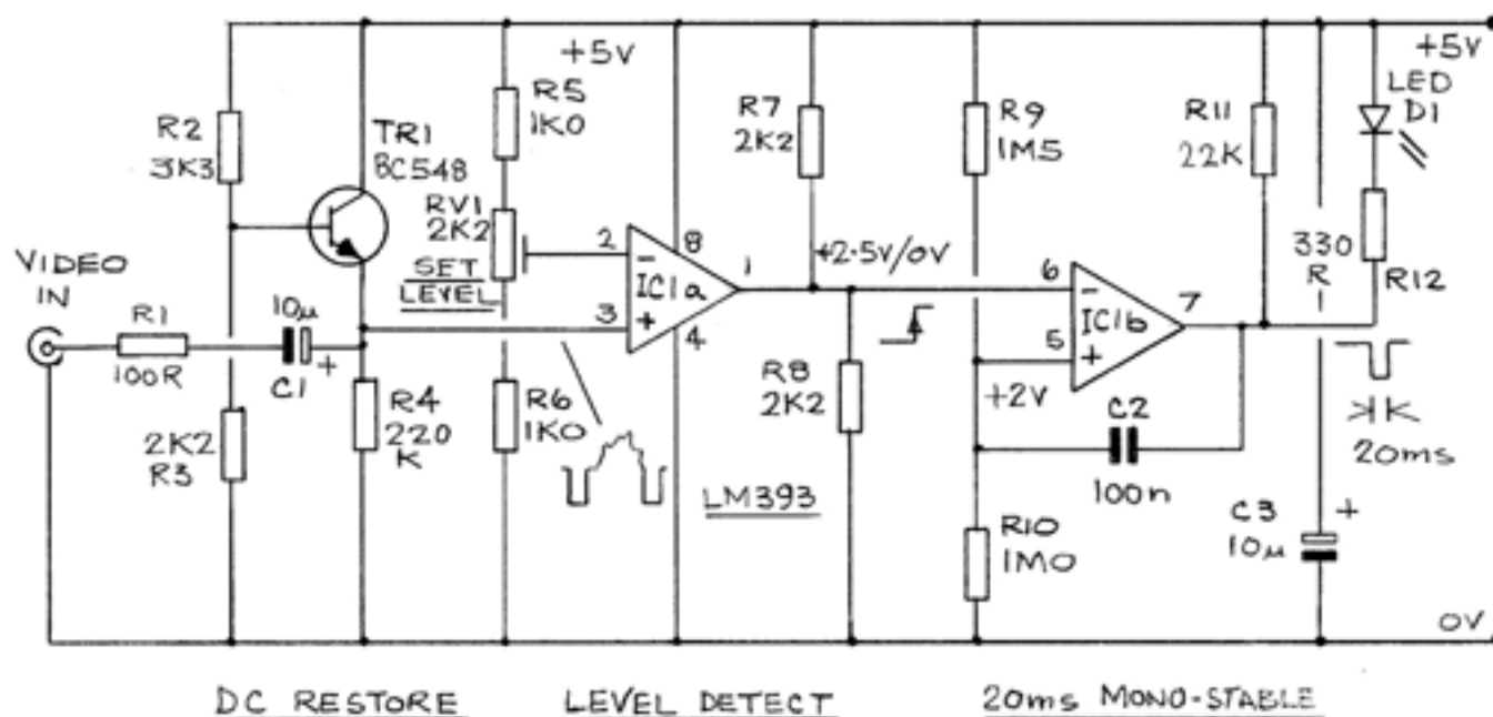
Fig.1. A Simple Peak Video Detector
