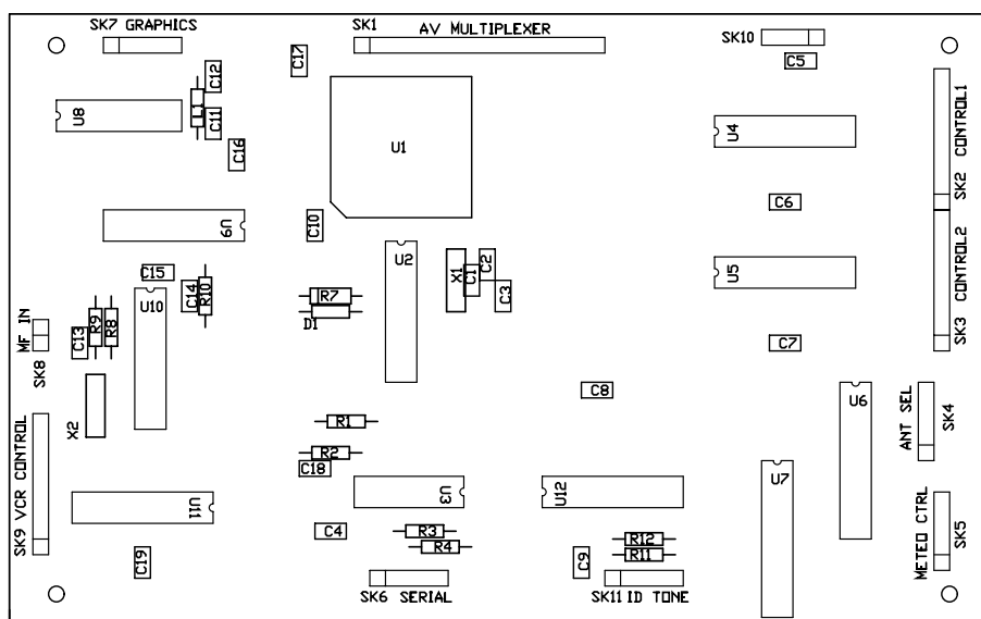
Component placements on the Sysproc board.
