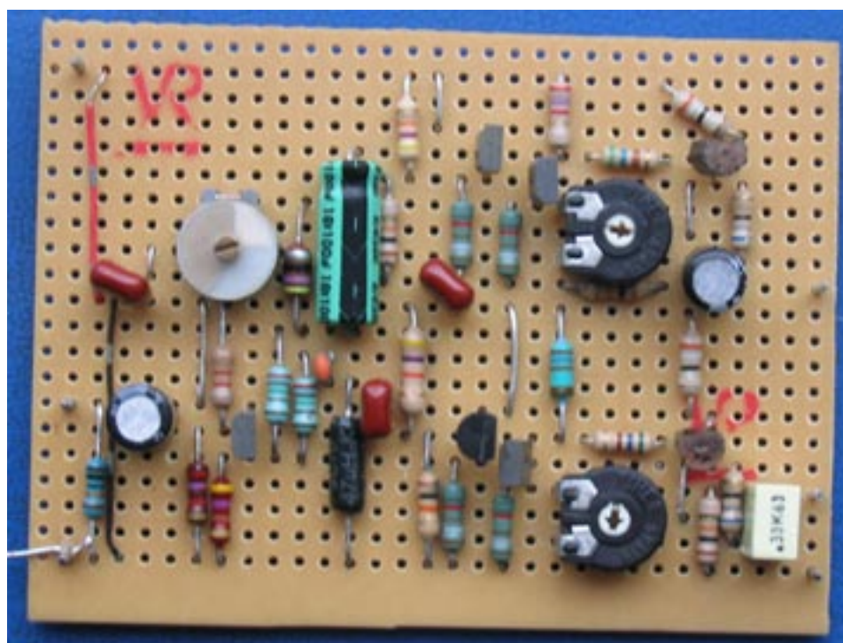
Veroboard layout.
